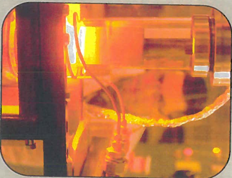
Dr. Travis Knight, co-principal investigator of both USC Nuclear CoEEs, works on a fluidized bed chemical vapor deposition coater to produce coated particle fuels for high temperature gas-cooled reactor applications.
