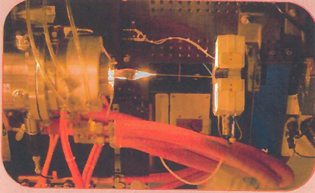
The birth of optical fiber: Drop of glass at 4,000 degrees Fahrenheit, in the process of making optical fiber. Clemson University is one of only a handful of universities in the world with industry-level capability to make optical fiber.
