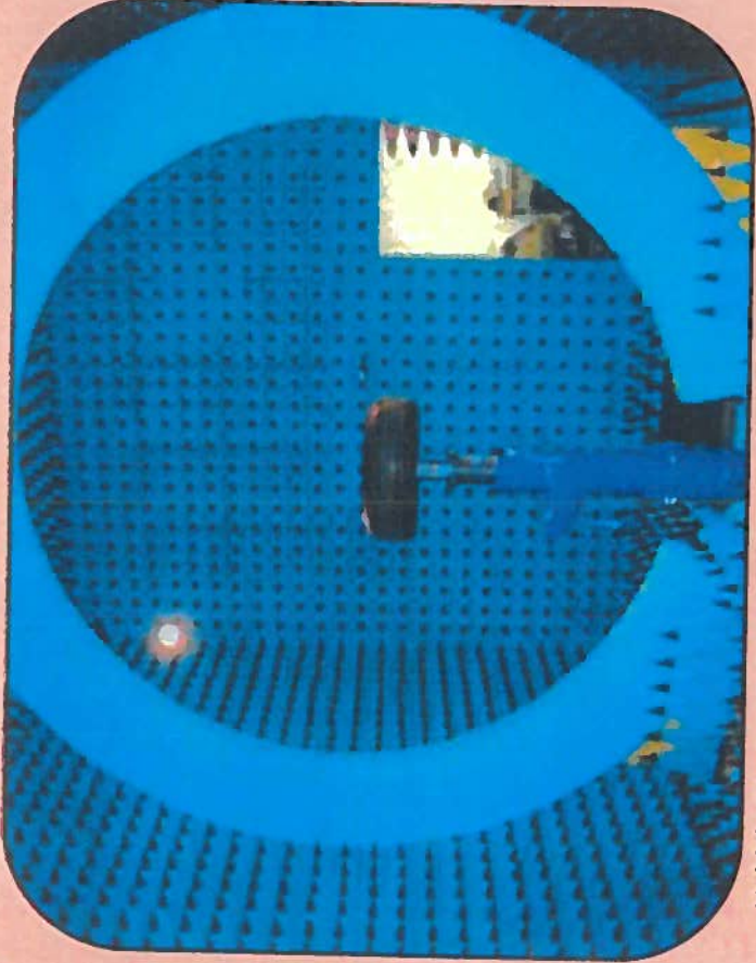
Vehicle Electronic Systems Integration Tire Antennae Project.
